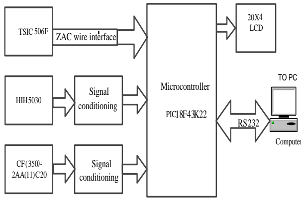
Fig. 1: Block diagram of the measurement system
